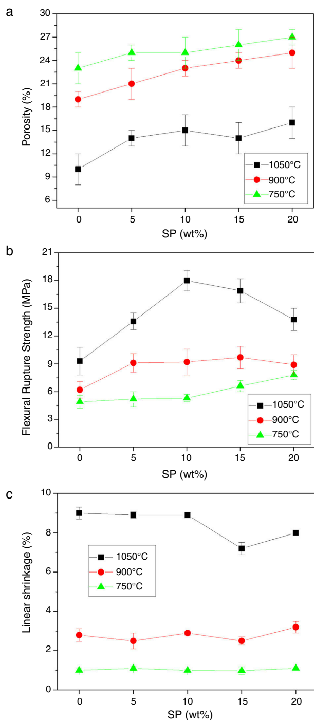
Fig. 3 – Porosity (a), flexural rupture strength (b) and linear shrinkage (c) of the clay ceramic as a function of the amount of the incorporated SP.
