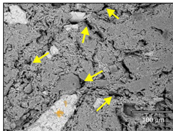
Fig. 4 – SEM micrograph of 20 wt% SP incorporated clay ceramic fired at 750 °C (pores indicated by arrows).
