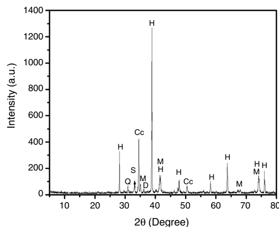
Fig. 1 – XRD pattern of the SPs: Cc = calcite; D = dolomite; H = hematite; M = magnetite; Q = quartz; and S = silvite.
