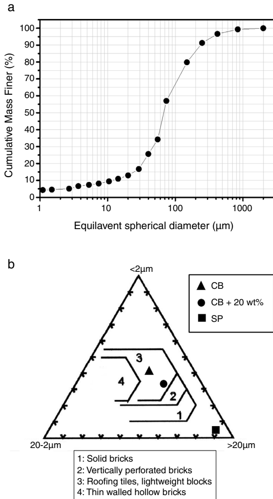
Fig. 2 – Particle size distribution of SP (a) and Winkler diagram showing regions of ceramic application in building construction (b).
