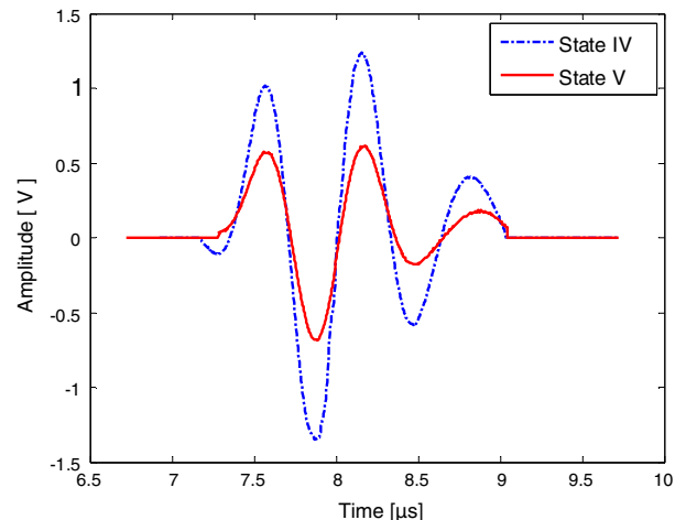
Fig. 3 – Time domain signal of second backwall echo in HP steel samples. A higher amplitude is observed for state IV and a larger attenuation for state V.
